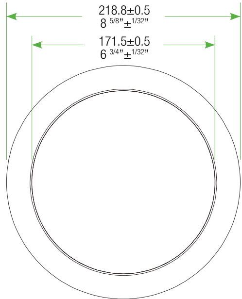
18W Trim ring
