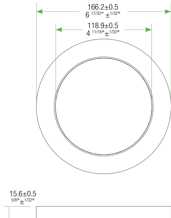
12W Trim ring
