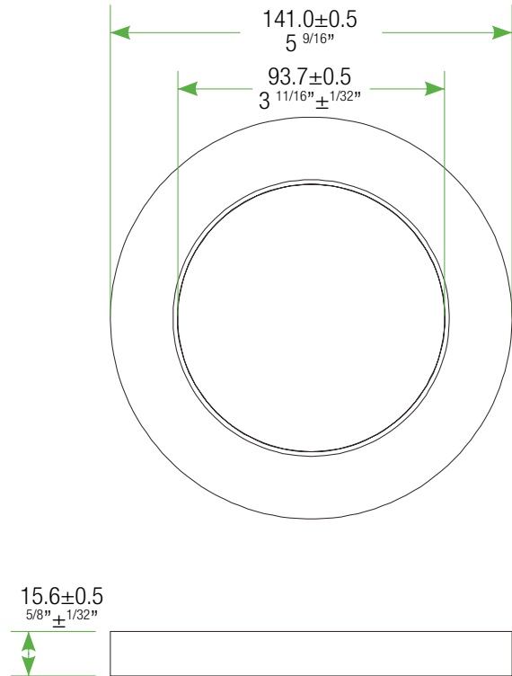
6W Trim ring
